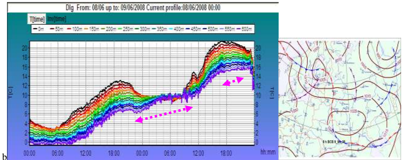
Fig.9. Temperature changes associated with a warm front passage (the pink arrow)
