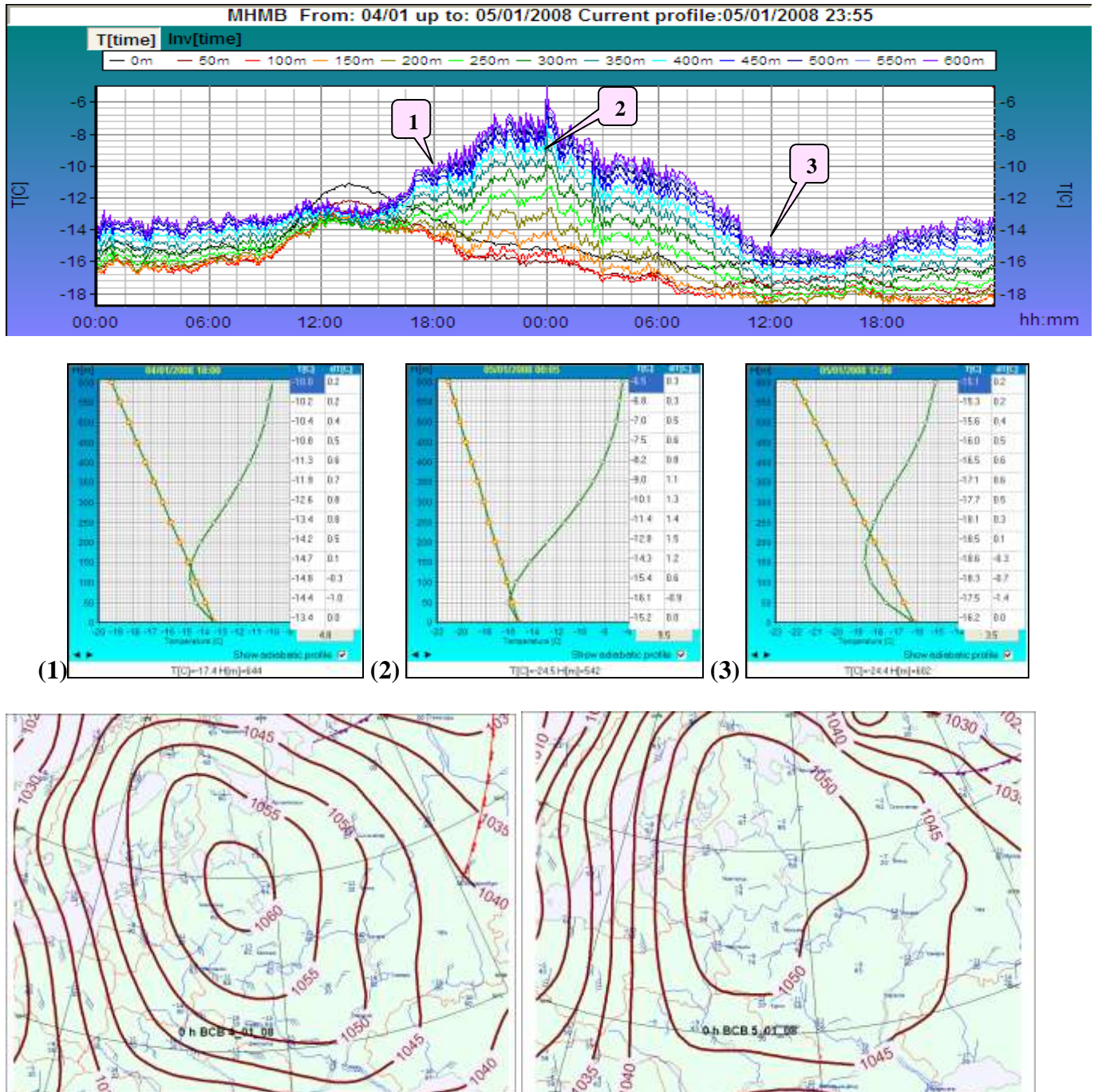
Fig.21. Inversion enhancement due to ordered anticyclone downdrafts.
