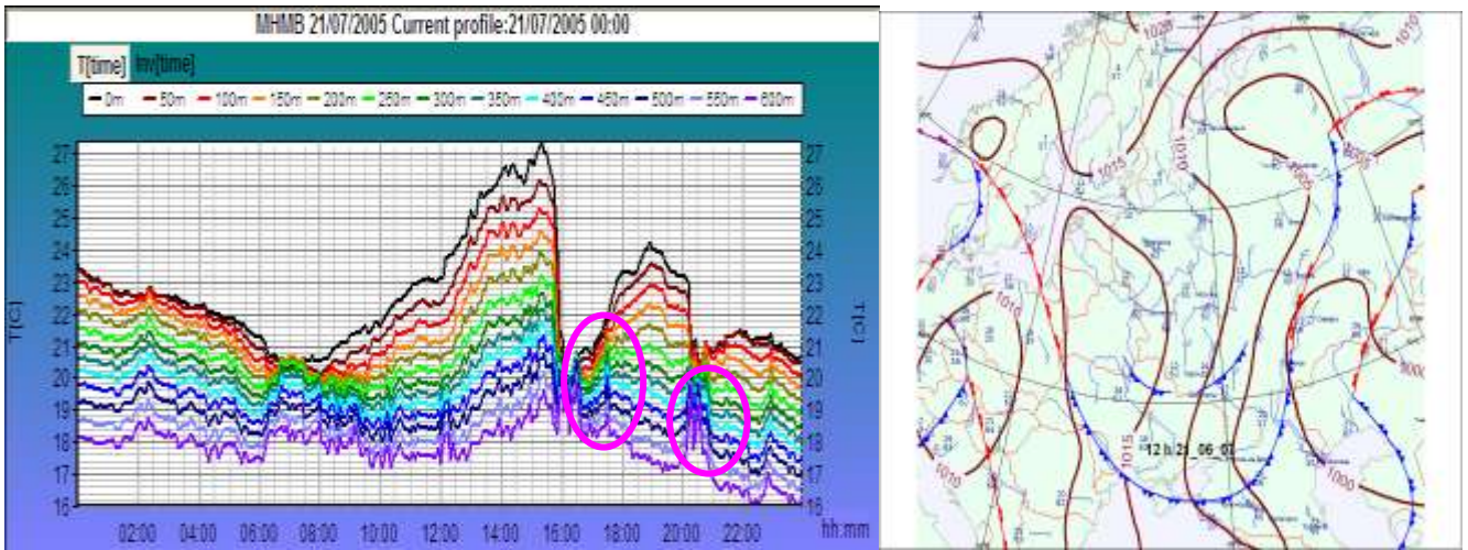
Fig.14. Thermal structure changes during the rain (pink contours) and the corresponding weather chart. It rained at about 16:00 and 20:00. Within the interval between the rains, the thermal structure of the lower atmospheric layer was rapidly restored: vertical temperature gradients exceeding a dry-adiabatic gradient were formed.
