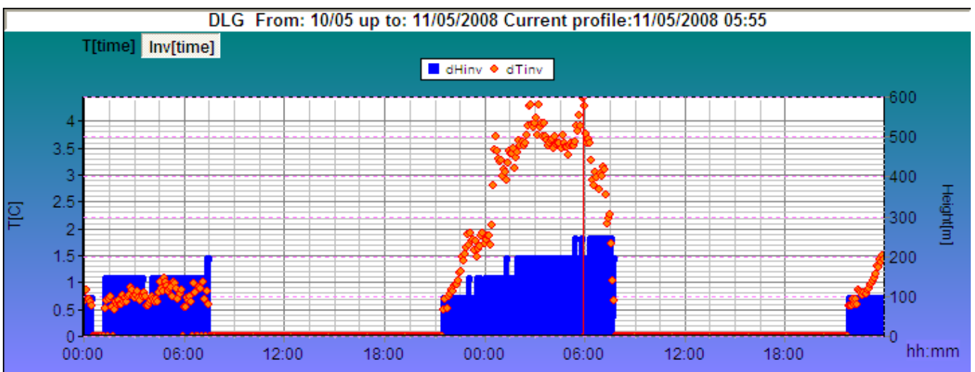
Fig.4. Temperature inversion characteristics. The duration of the 10 May nighttime inversion was 7.5 hours with the lower boundary at 0 m, the upper boundary at 150 m, and a magnitude of 0.8°C (maximum 1°C). The 11 May inversion formed in the evening of the day before (21:00) and persisted till 07:00, hence a 10-hour duration. The characteristic magnitude of inversion on 11 May was 3.5°C (maximum 4.5°C) with the characteristic upper boundary at 200 m (175 m on average).
