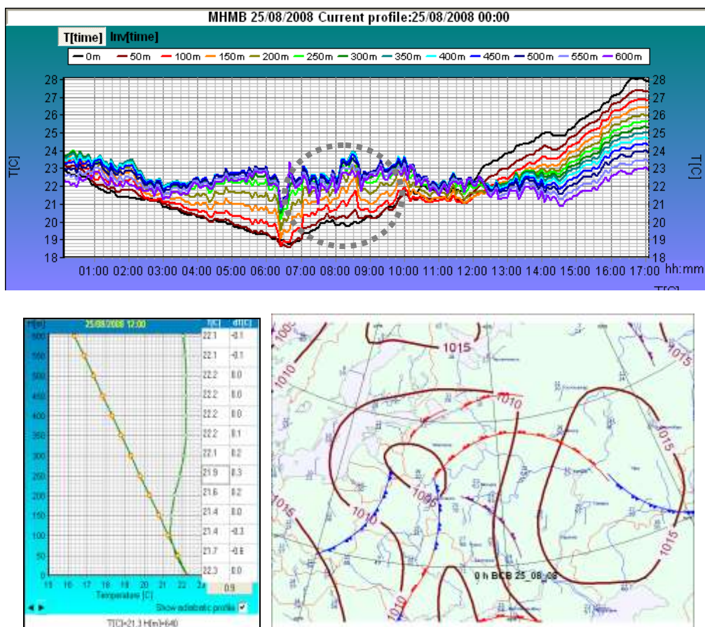
Fig. 24 An abnormal diurnal variation of thermal stratification (grey contour) caused by the advection of polluted air from forest and steppe fires in a warm cyclone sector. August 2008. An abnormally stable
