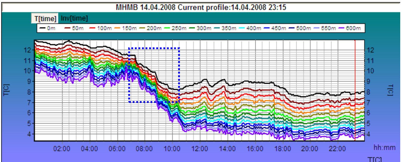
Fig.8. Temperature changes in the zone of a secondary cold front (square contours):
