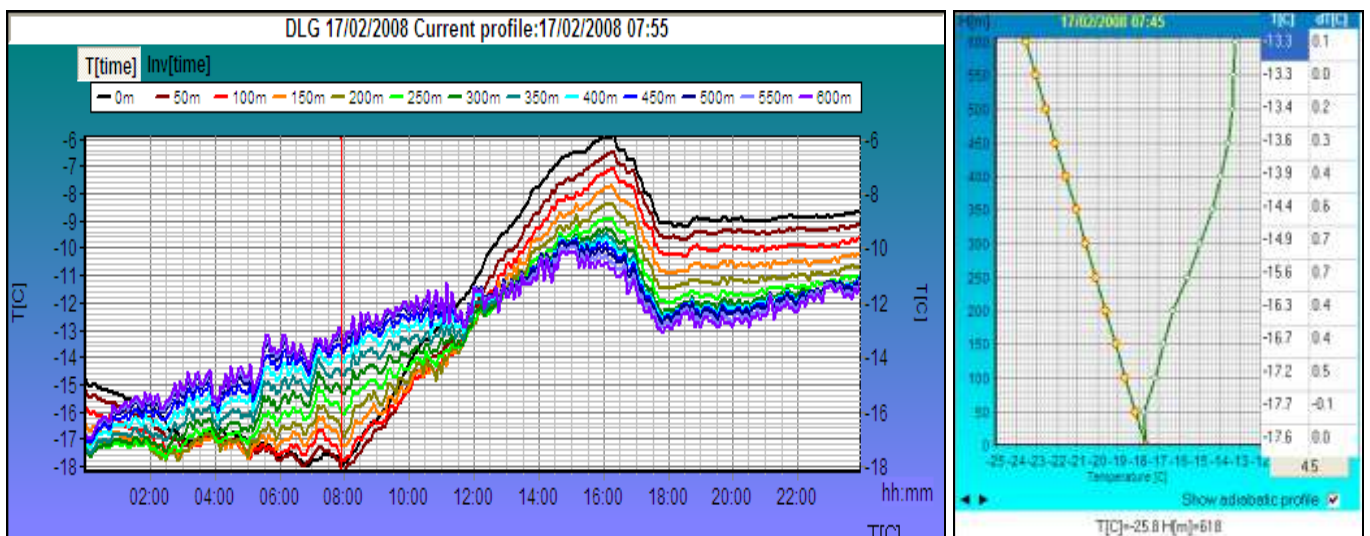
Fig. 19. Frontal (advection) inversion in a warm front (Fig. 9, the chart). As night temperature decreases at the surface, at 600 m it rises: in the period between 00:00 and 08:00: surface temperature dropped by 3°C, while in the upper measurement layer portion, a 4°C increase was observed, the temperature continuing to rise at a 600-m level during the next 10 hours.
