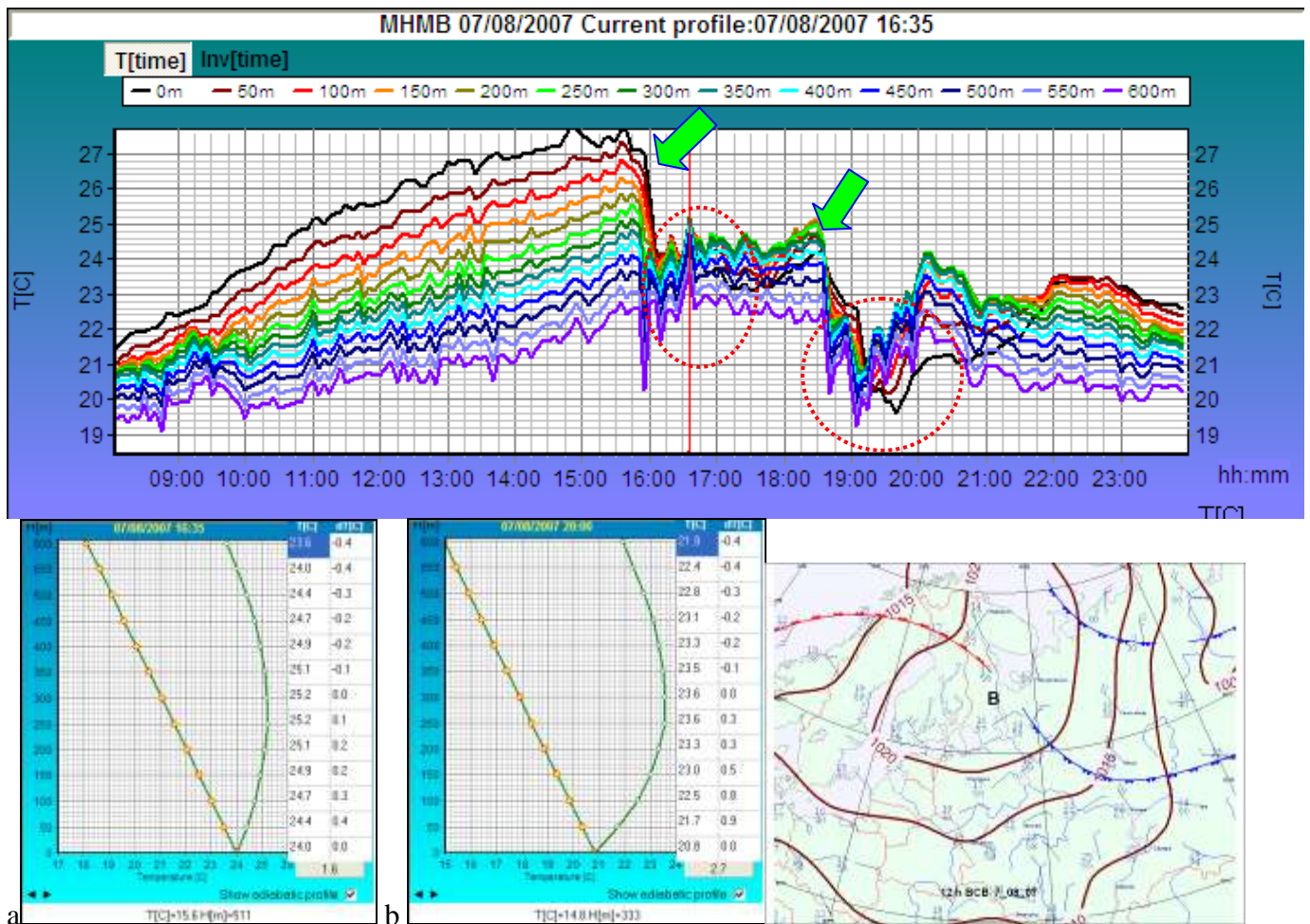
Fig.22 Evaporation inversion (showed by red contours in the top picture) after 7 August daytime shower rain. In the pictures below: temperature inversion a) at 16:35 and b) at 20:00. The top picture presents two fragments with sharp temperature changes typical of a convective precipitation period (green arrows indicate the beginning of showers). During the first shower, which lasted for less than an hour, the temperature at 600 m changed by nearly 3°C within 10 min., signifying intensive vertical mixing. After the rain, surface inversion formed due to evaporative surface cooling persisted for about 2 hours in an unusual daytime period, its magnitude nearly reaching 2°C. After the second rain, evaporation inversion persisted during the period from 19:00 to 22:00; the nighttime inversion, enhanced by natural cooling, exceeded the daytime one.
