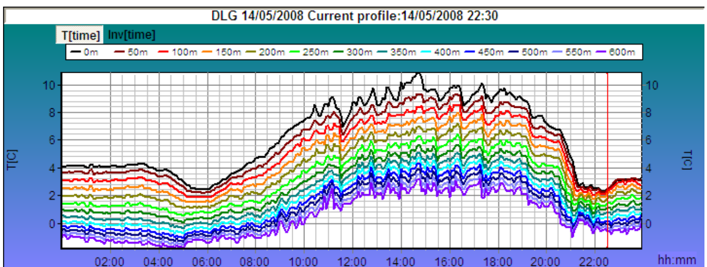
Fig.13 Temperature changes due to varying cloud amount during a warm season.
