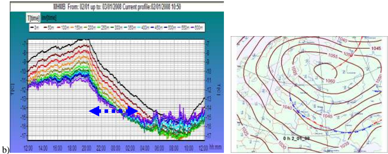
Figure 7. Passage of a cold atmospheric front in winter (a blue arrow).
