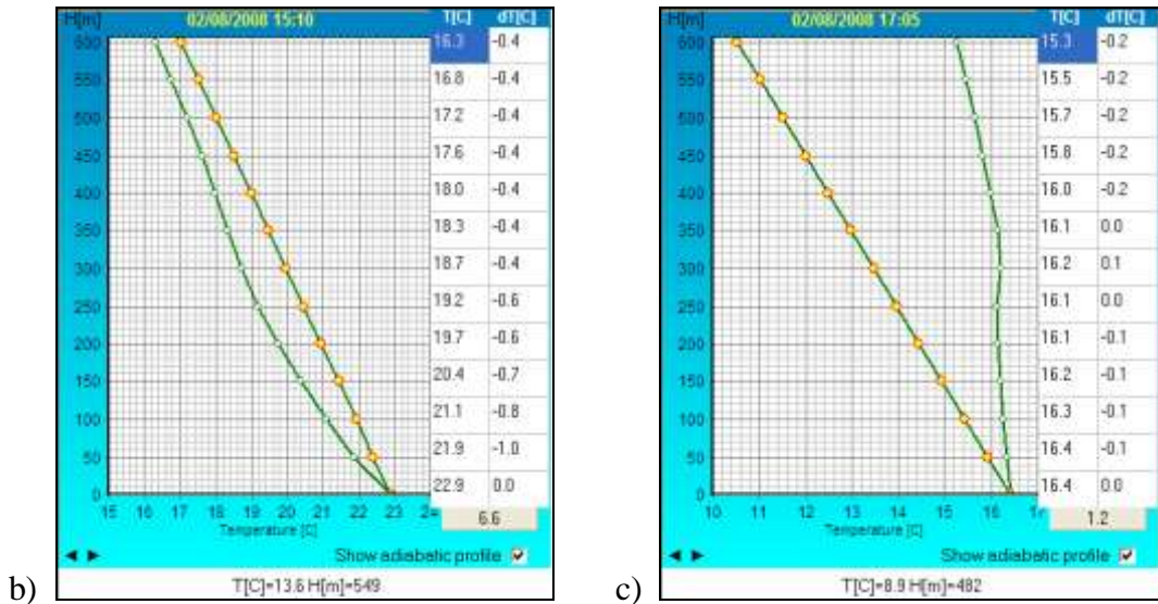
Fig.6.: (a) Passage of a cold atmospheric front in summer (blue arrow, 16:30-21:00); (b) Thermal stratification ahead of the front (highly unstable), and (c) The zone of front (virtually isothermal).
