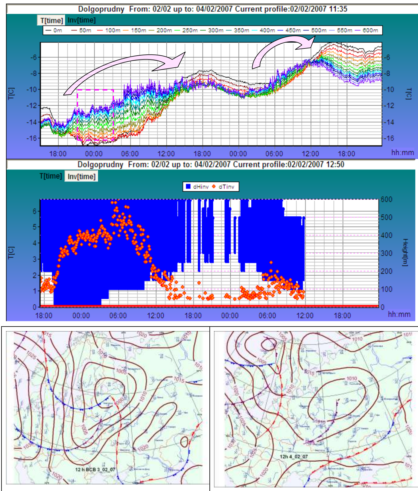
Fig. 5. An example of mixed advection-radiation temperature inversion and weather map for one episode. The first heat wave (the pink arrow in the upper picture) persisted for 12-14 hours with a temperature rise by about 5^{\circ}\text{C} throughout the measurement layer. Against the background of the nighttime temperature increase with low wind the lower inversion boundary descended to the ground due to
