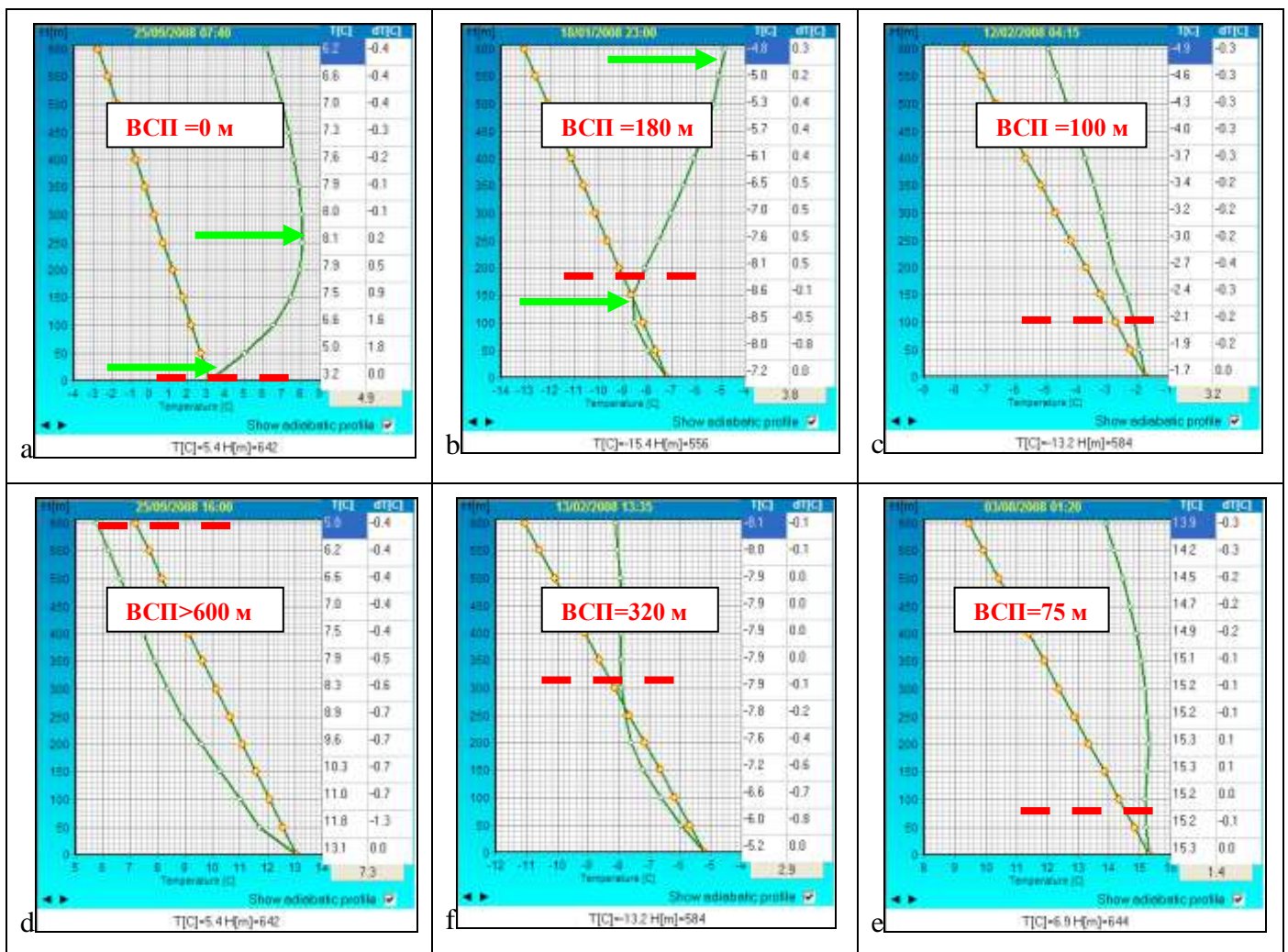
Figure 2 – MLH for different types of thermal stratification (red dashed line). Green arrows show temperature inversion boundaries.
